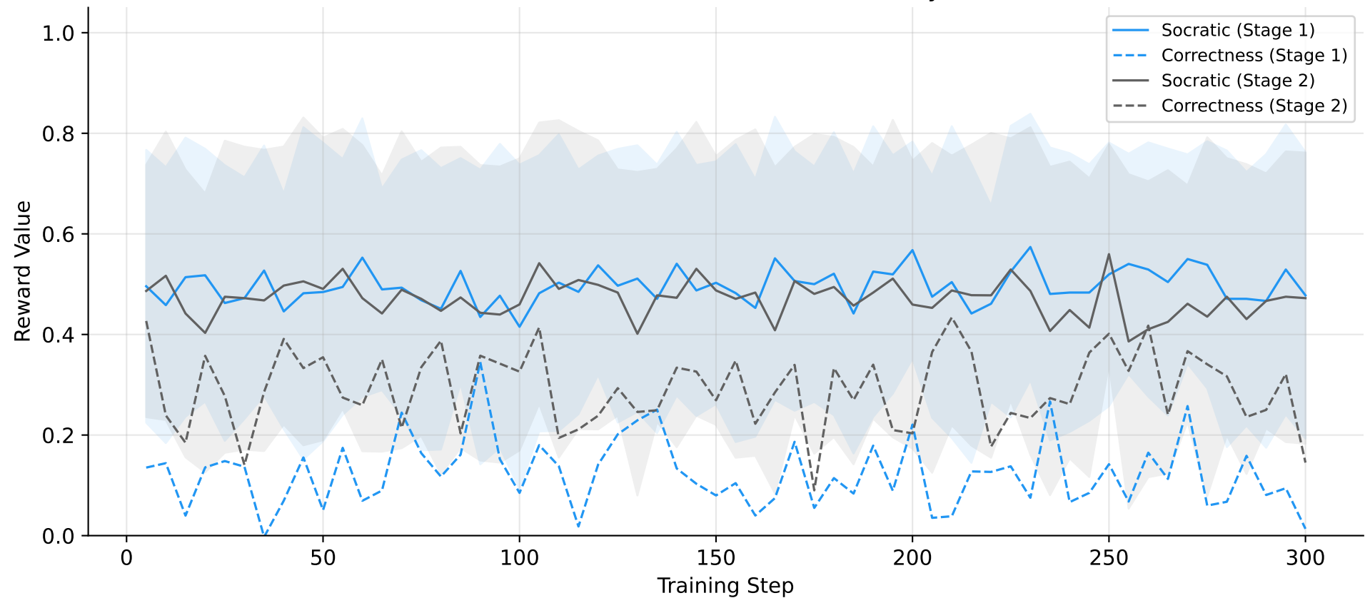
GSPO: Socratic vs Correctness Reward Dynamics
